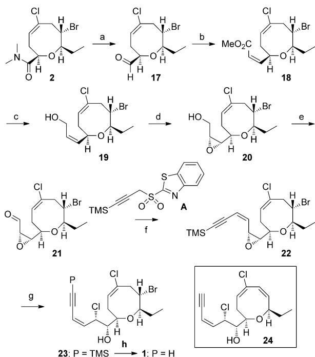
Scheme 5. Completion of the synthesis: a) DIBAL-H (2 equiv), n\text{BuLi} (2 equiv), THF, 0 °C, 10 min, then RT, 50 min, 83 %; b) (\text{CF}_3\text{CH}_2\text{O})_2\text{POCH}_2\text{CO}_2\text{Me} , KHMDS, [18]crown-6, THF, –78 °C, 15 h, 71 %, Z/E = 10:1; c) DIBAL-H, toluene, –78 °C, 30 min, 96 %; d) \text{VO}(\text{acac})_2 , t\text{BuOOH} , benzene, 40 °C, 15 h, \alpha/\beta = 2.3:1 , 70 % total yield; e) DMP, \text{NaHCO}_3 , \text{CH}_2\text{Cl}_2 , RT, 5 h, 96 %; f) A , KHMDS, THF, –78 °C, 30 min, 53 %, Z/E = 16:1; g) \text{TMSCl} , DMAP, \text{EtOAc} , RT, 3 h, 76 %; h) TBAF, acetic acid, THF, 0 °C, 30 min, 90 %. DMP = Dess–Martin periodinane, TMS = trimethylsilyl, DMAP = 4-dimethylaminopyridine, TBAF = tetra- n -butylammonium fluoride.
